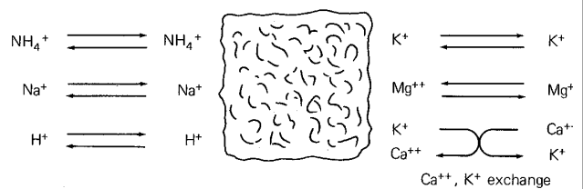
Figure 5-5 Cation exchange on a clay particle. The lower right reaction illustrates replacement of K + by Ca ++ .
