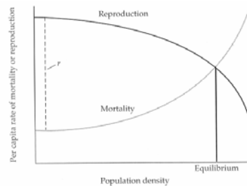
Figure 8.8 Density dependence stems from relationships between population density and per capita rates of birth and death. The difference between these rates at a small population size is the intrinsic rate of natural increase, r , and the density at which these rates are balanced is the equilibrium population size.
