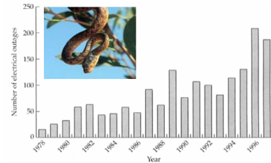
Figure 9.2 Annual electrical outages caused by the invading brown tree snake on Guam. (Modified from Fritts 2002.)
