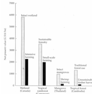
Figure 6.21 Economic value (net present value) from managing ecosystems in sustainable ways (gray bars) is higher than for unsustainable uses of that same ecosystem type (black bars). (Modified from Botsford et al. 2002.)
