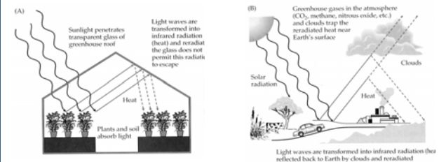
Figure 10.1 The greenhouse effect. Earth's atmosphere already serves as a greenhouse that warms Earth's surface (A), but human influences are increasing this effect (B). About 70% of UV wavelengths pass through Earth's atmosphere, where about 30% are reflected. Burning of fossil fuels in industry, as automobiles, and buildings, as well as deforestation give off \text{CO}_2 to the atmosphere that enhance the greenhouse effect. In addition, methane from swamps, rice paddies, and cattle enter the upper atmosphere and trap heat. (From Primack 2004.)
