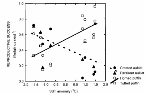
Fig.4. Reproductive success of planktivorous auklets and piscivorous puffins in relation to SST anomaly during 1 July – 30 August in Tauskaya Bay.
