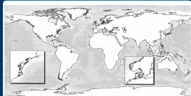
Figure 6.16 World distribution of hypoxic or "dead zones" is correlated to position of watersheds that have greatly enhanced nitrogen inputs, and to major cities. (Modified from Burke et al. 2000.)
