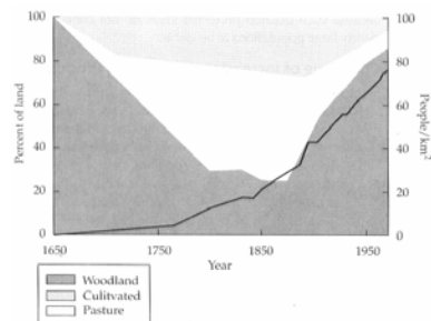
Figure 6 Beginning in the mid-1600s, the landscapes of New England were largely converted to pasture and croplands, but with the industrial revolution were abandoned and reforested until the present day. Population density (black line) increased over the same period, as people moved to cities from the countryside. (Modified from Foster 2002.)
