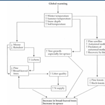
Figure A Effects of climatic warming on the biotic interactions likely to influence forest composition in northern Finland, Norway, and Sweden. (Modified from Niemelä et al. 2001.)
