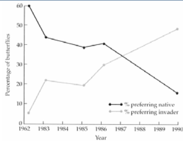
Figure 9.8 Percent of Euphydryas editha (a native checkerspot butterfly) preferring to oviposit on the native plant Collinsia parryiflora (black line) versus the introduced Plantago lanceolata (gray line) over time in Nevada. (Modified from Singer et al. 1993.)
