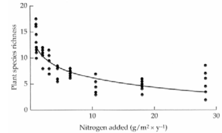
Figure 6.15 Plant species richness declines along a nitrogen gradient in a prairie ecosystem at Cedar Creek, Minnesota. (x-axis is the rate of nitrogen addition plus 1). Each point represents the average of data collected in 1995 and 1996. (Modified from Haddad et al. 2000.)
