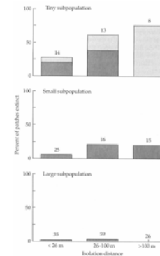
Figure 7.15 Extinction rates were highest in small, isolated patches (subpopulations) of the annual plant Clarkia concinna (Onagraceae). White portions of bar denote patches, in which individuals had no, or low, reproductive success, and dark gray portions denote patches that experienced a catastrophe (e.g., a flood); sample sizes are above bars. (From Groom 1998.)
