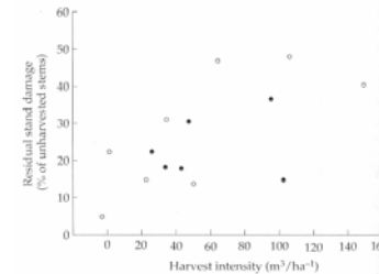
Figure B Variability in harvest intensities ( \text{m}^3/\text{ha}^{-1} ) and incidental damage to the residual stand (percentage of unharvested trees) across the tropics. Open symbols are areas in which harvesting was planned and controlled; closed symbols are areas in which harvesting was carried out in a conventional way (typical for the region, generally with little planning and control over operations). (Modified from Pinard et al. 2005.)
