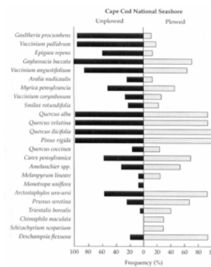
Figure 6 The understory flora of woodlands that had once been cultivated for agriculture (plowed) differs from that found in sites that had always been woodlands (unplowed) in the Cape Cod National Seashore, MA. In this region, as in much of New England, lands were cleared of trees to make way for agriculture, plowed, and beginning in the nineteenth century, abandoned and allowed to reforest. Both plowed and unplowed sites have been forested and managed since the late nineteenth century, yet a century after their use, the flora clearly differs. There are three groups of species represented, (1) species (especially ericaceous shrubs) that are more abundant in former woodlands that were eliminated by agriculture and have failed to reestablish, (2) weedy species that established well in agricultural sites and persisted there, but that are incapable of establishing widely in intact forest areas, and (3) species that are excellent dispersers and establish readily in any site. (Modified from Foster et al. 2003.)
