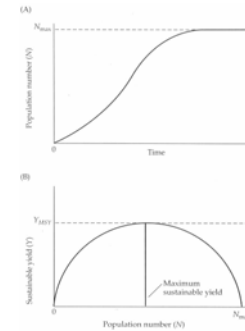
Figure 8.9 (A) Logistic population growth of a population up to a maximum population size, N_{max} . (B) Sustainable yield, Y (surplus production) against population size for the logistic case shown in (A). The maximum sustainable yield ( Y_{max} ) occurs at 50% of the maximum population size.
