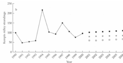
Figure 8.14 Projected annual strandings for Kemp's ridley sea turtles based on three potential levels of compliance by shrimpers in using turtle excluder devices in their nets. Black squares = compliance at 2000 levels, gray squares = 50% improved compliance over 2000 levels, and open squares = full compliance. Fluctuations in strandings reflect variation in compliance and sea turtle abundance in areas where shrimp fisheries are most active. (Modified from Lewison et al. 2003.)
