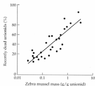
Figure 9.4 Percent of native unionid mussels recently dead as a function of the relative wet weight of introduced European zebra mussels ( Dreissena polymorpha ) attached to their shells. Note log scales. (Modified from Ricciardi 2003.)
