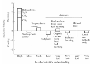
Figure 10.5 Estimates of strengths of radiative forces on global energy budget. Radiative forcing is in \text{watts}/\text{m}^2 . Positive forces (above zero) warm Earth's surface; negative forces (below zero) cool Earth's surface. (Modified from IPCC 2001a.)
