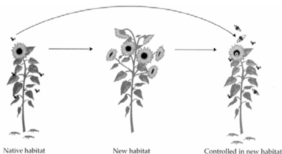
Figure A Invasive species are often those that escape their herbivores from their native habitat in a new habitat, and grow at a much higher rate as a result. Biocontrol attempts to halt this rapid growth by introducing the herbivore(s) that kept the plant in check into its new habitat.
